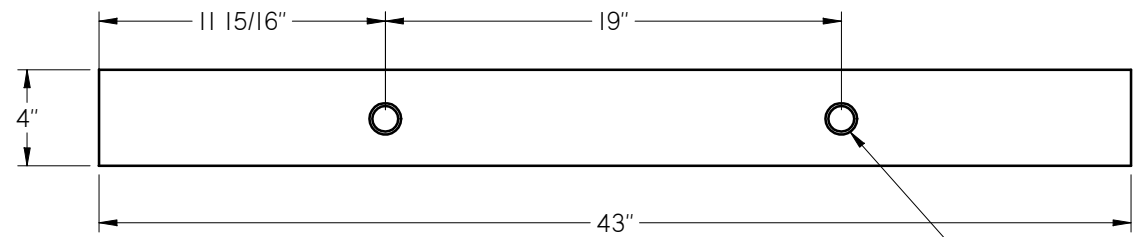
Arch push plates (2)
