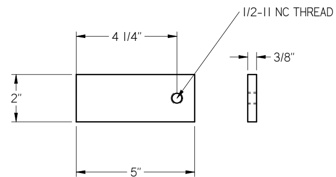
DOOR RAIL TAB(2) WITH HOLES
