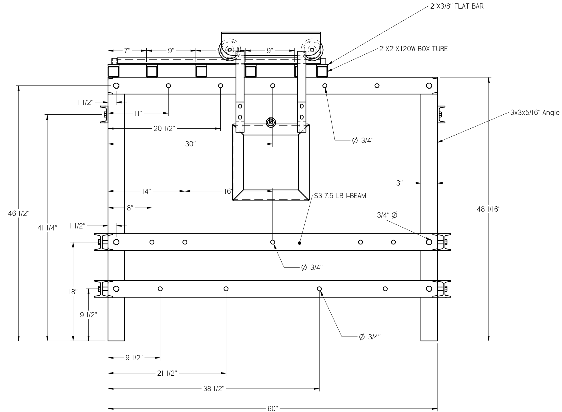
FRONT VIEW
