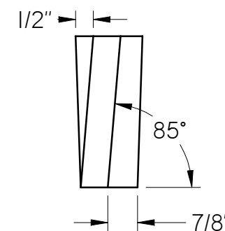
THERMOCOUPLE BRICK
