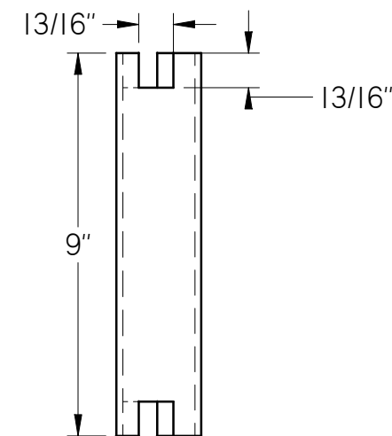
THERMOCOUPLE BRICK
